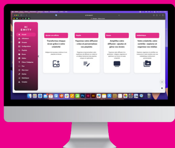
E-MANAGER
